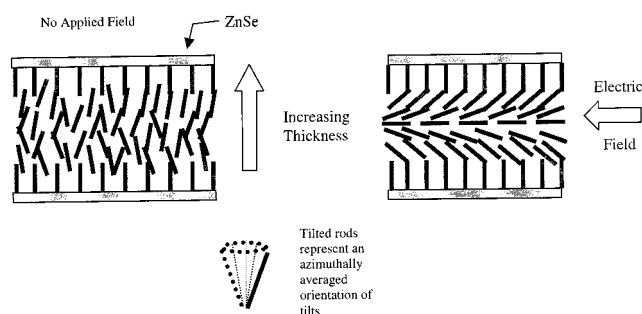
Figure 7. Schematic model of the initial and the transition to the electric field-induced orientation of 5CB within a single nanocavity. The orientations shown are not a quantitative depiction of the canted organization of the 5CB molecules present in the absence of an applied electric field. It is not known if the tilt anisotropy extends completely to the cell wall. The tilt anisotropy noted reflects an average measured over the dimensions of the cell probed by the beam.
