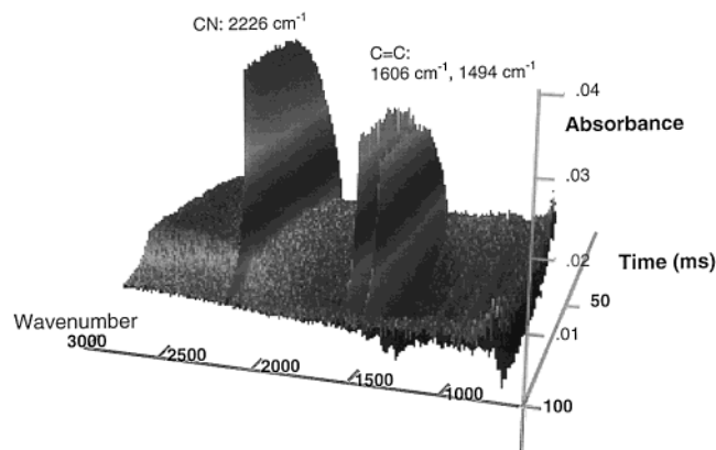
Figure 8. Three-dimensional time-resolved spectrum of 5CB. Prominent modes increase with time after the applied pulse of 12.6 V, plateau when maximum orientation in the applied field is achieved, and then relax back to the preperturbed orientation.
