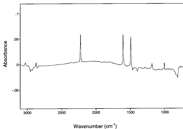
Figure 4. Infrared difference spectrum of 5CB taken with light polarized perpendicular to the IDA bands. The spectrum is the ratio of the 5CB-filled 40 nm cell held at 15 V to the same cell held at 0 V. Positive peaks show modes that have oriented perpendicularly to the IDA bands while negative peaks represent vibrational modes that have reoriented parallel to the IDA bands upon application of the electric field.
