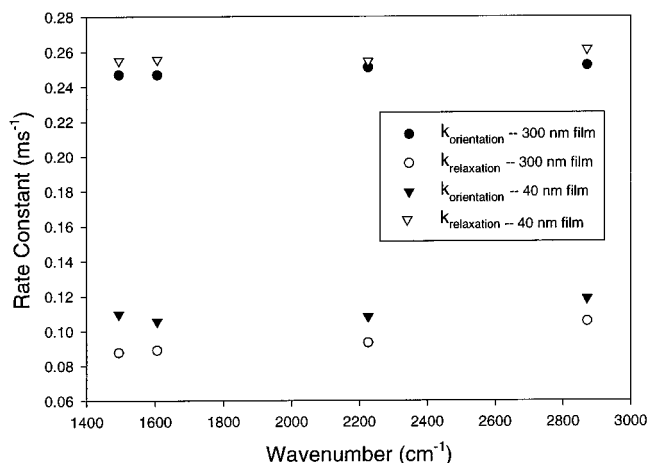
Figure 11. Rate constants for the orientation and relaxation of 5CB under an applied electric field determined from the fits shown in Figure 10. The rate constants for the 40 nm film are represented by triangles showing a larger k for relaxation and a smaller k for orientation. The rate constants for the 300 nm film are represented by circles and the relationship between rate constants is reversed from that of the 40 nm film with k for orientation being larger than k for relaxation.
