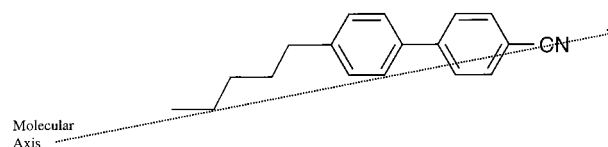
Figure 1. Structural diagram of 4- n -pentyl-4'-cyanobiphenyl (5CB). The vector overlaying the structure of 5CB indicates the molecular axis used to define the orientation of the molecule.
