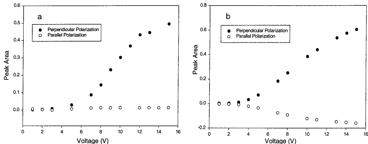
Figure 6. Peak area versus applied voltage for the CN stretch at 2226 cm -1 : (a) 40 and (b) 300 nm film.
