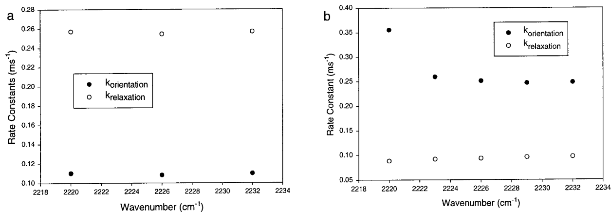
Figure 12. Rate constants measured across the width of the 2226 \text{cm}^{-1} vibrational mode: (a) 40 and (b) 300 nm film. Kinetic inhomogeneity is seen in the orientation of the 5CB in the 300 nm film while the other processes appear to be kinetically homogeneous.
