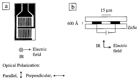
Figure 3. (a) Top view of an interdigitated electrode array (IDA) with optical polarization defined relative to the electrode fingers. (b) Cross section of thin-layer confinement cell with bands 15\ \mu\text{m} wide and 15\ \mu\text{m} from neighboring bands. The height of the IDA defines the thickness of the thin film. Shown here is the thinnest cell, 40 nm thick.
