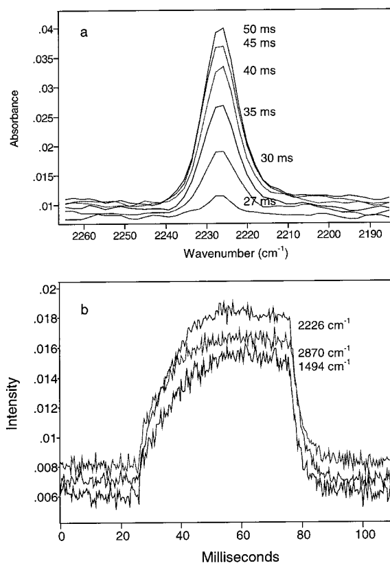
Figure 9. (a) Difference peaks for 2226 \text{cm}^{-1} at various times after a 12.6 mV pulse is applied. This cross section of Figure 7 illustrates the time scale for the orientation of 5CB in the electrooptical cell. (b) Intensity traces for representative vibrational mode difference peaks of 5CB upon application and removal of an electric field across the 40 nm thin film. These traces can be fit with rising and decaying exponential functions to determine the rate constants for the orientation and relaxation of 5CB.
