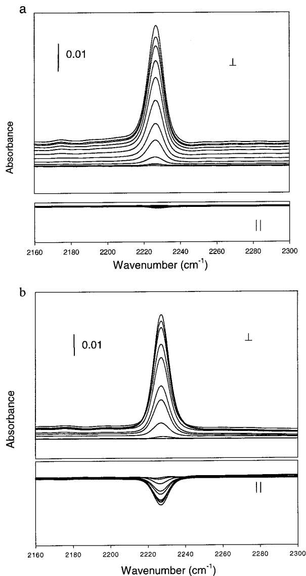
Figure 5. Difference peaks of the CN stretch for both parallel and perpendicular polarization as voltage is increased in increments from 1 to 15 V. Zero volts is used as the reference spectrum. (a) The 40 nm IR cell. The peaks with greatest intensity occur at the highest applied voltage (15 V) due to increased anisotropy induced by the applied field. No change is seen in the parallel polarization. (b) The 300 nm film of liquid crystal. Like the 40 nm film, the intensity in the perpendicular direction increases with increased voltage. However, in this thicker film, the intensity decreases when probed with light polarized parallel to the IDA fingers.
